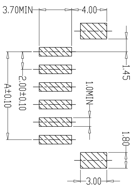
PCB LAYOUT
