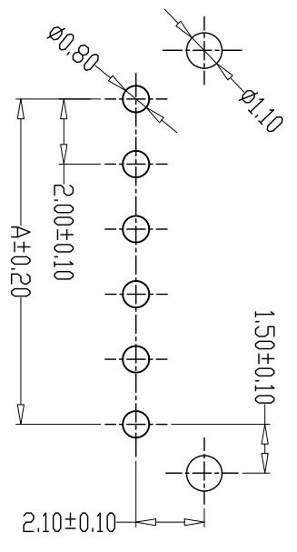
PCB LAYOUT
